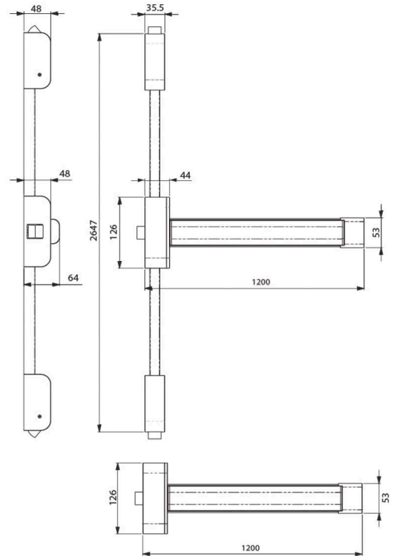
Technical drawing applicable PHDT50, PHDT55, PHDT57
